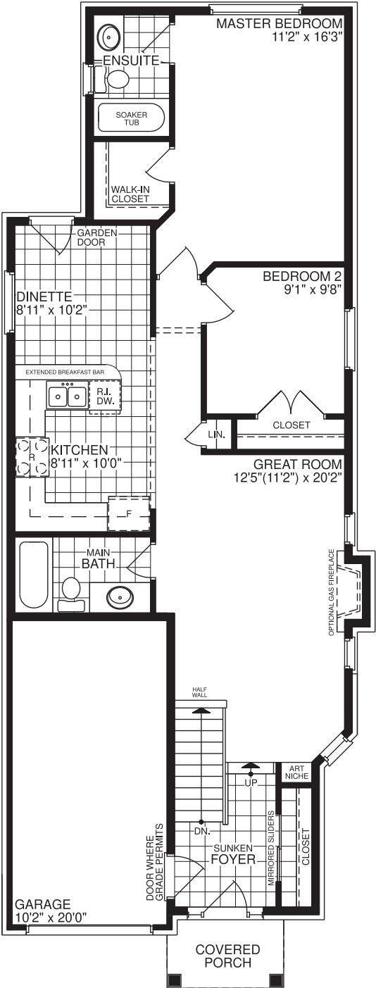
FIRST FLOOR PLAN ELEVATION A
